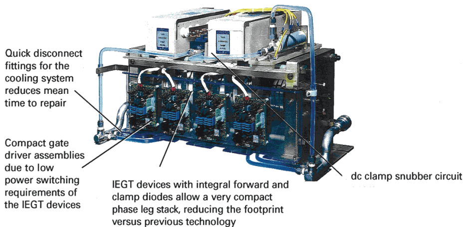
TM-70 Phase Leg Assembly
