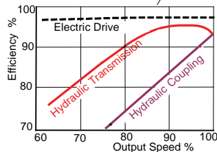
Figure 2. Hydraulic Transmission Efficiency
