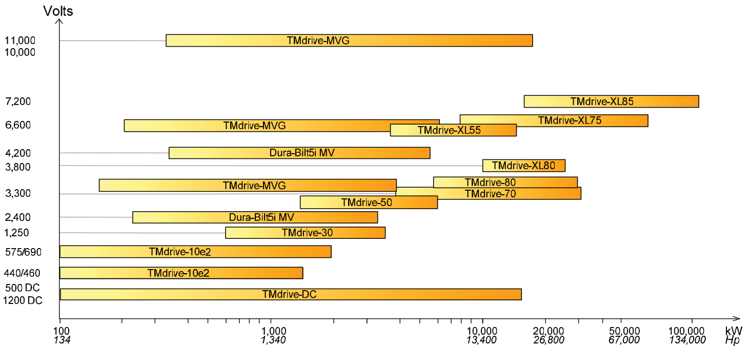
TMdrive-70
