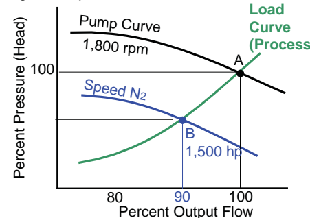
Fig. 4 Pump Performance Chart & Load Curve
