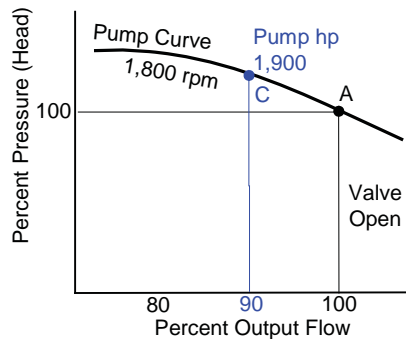
Fig. 1 Pump Performance Chart & Load Curve
