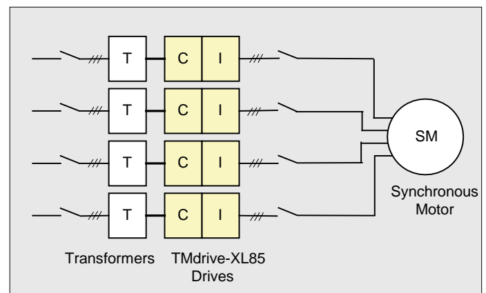
Simplified Block Diagram of Redundant VSD
