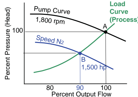
Fig. 3 Pump Performance Chart & Load Curve
