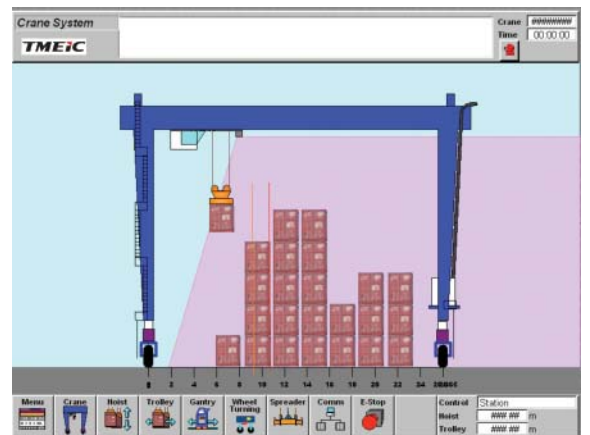
Maxview Smart Move system on an RTG Crane
