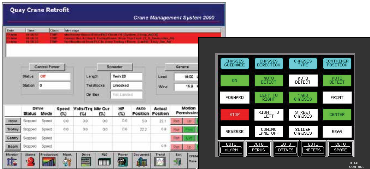
Two HMIs for Crane Monitoring and Diagnostics
