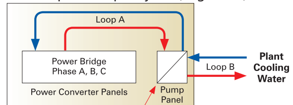
Liquid-to-Liquid Exchanger
