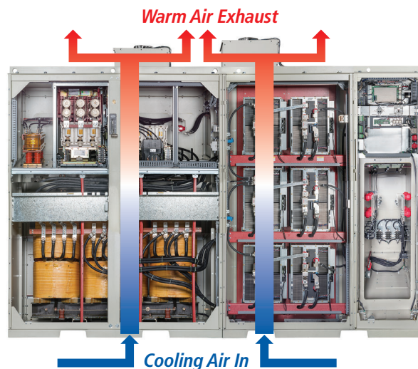
Figure 3. Typical air-cooled VFDs and air flow
