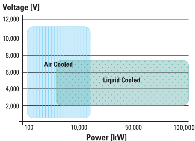
Figure 1. Power vs. voltage for air- and liquid-cooled VFDs
