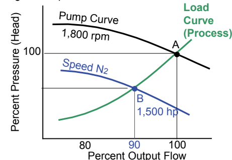
Fig. 4 Pump Performance Chart & Load Curve
