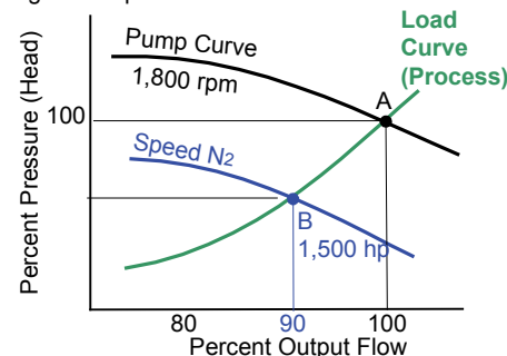
Fig. 3 Pump Performance Chart & Load Curve
