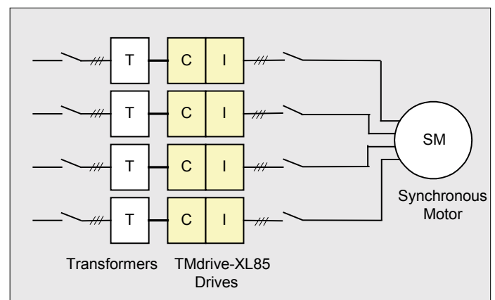
Simplified Block Diagram of Redundant VSD
