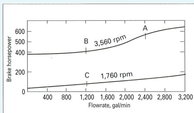
Typical pump head, flow, speed & power characteristics
