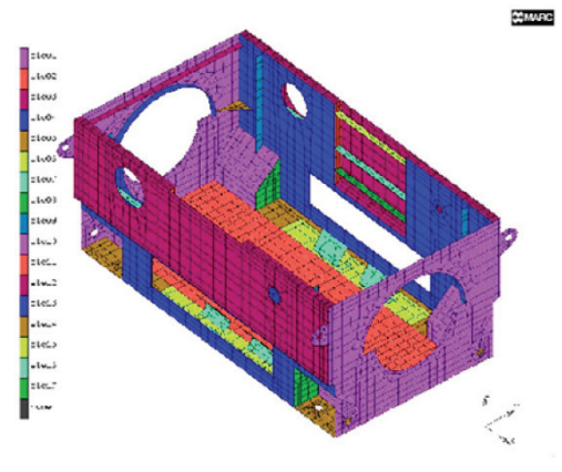
FEM Natural Frequency Analysis
